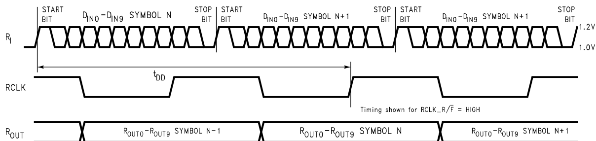
Figure 5. Deserializer Delay
