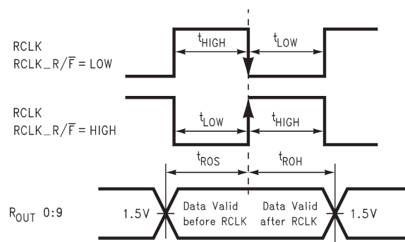
Figure 5. Deserializer Delay
